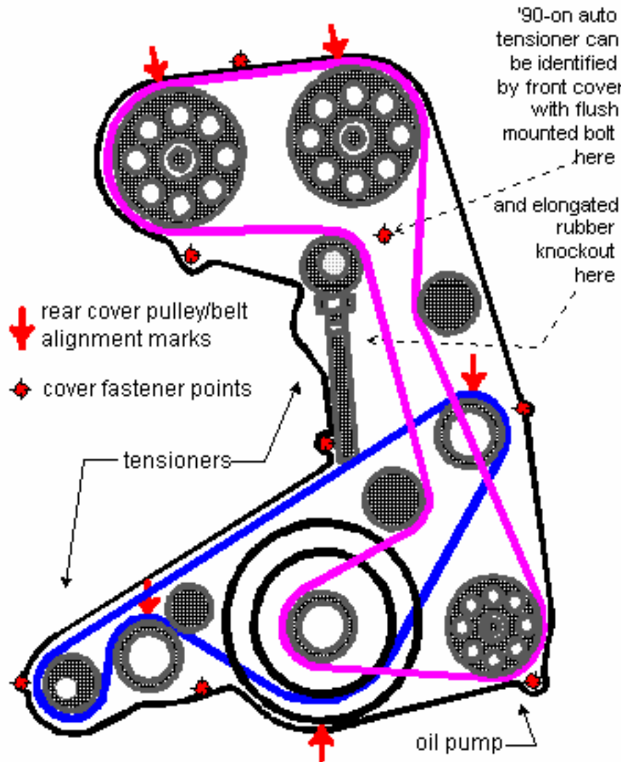
Later B234F with Automatic Tensioner
