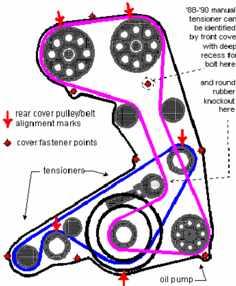
Early B234F with Manual Tensioner
